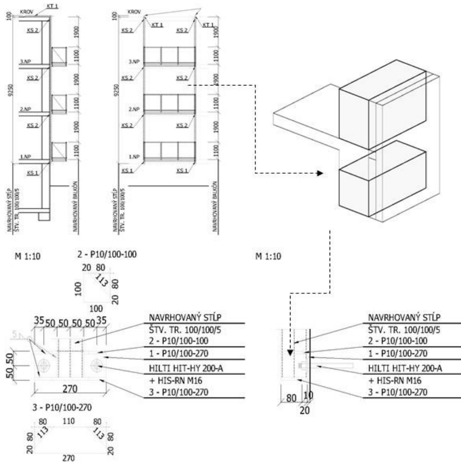
Fig. 3: Static solution and the principle of anchoring the overhanging loggias
