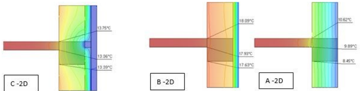
Fig. 4: 2D temperature profile for 3 variants
