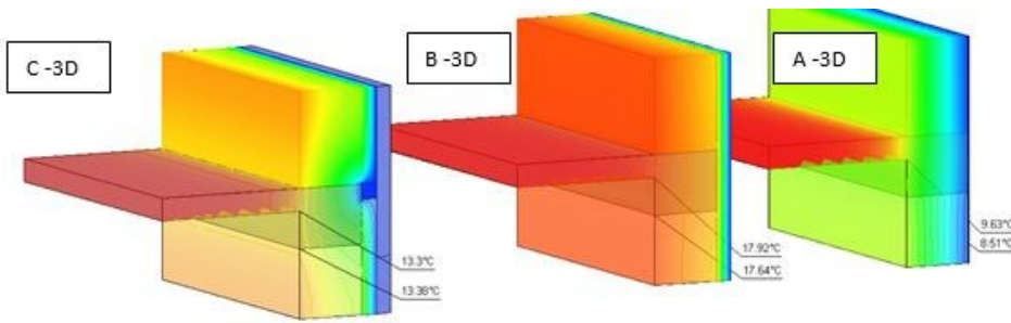
Fig. 5: 3D temperature profile for 3 variants
